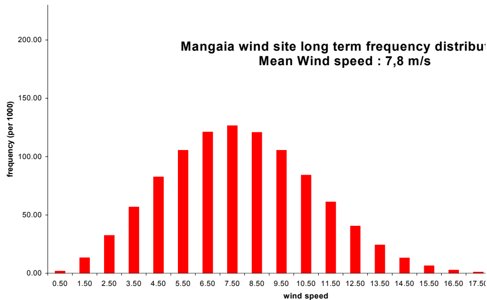
Figure B-1 - Mangaia Wind Site, Long Term Frequency Distribution. Mean = 7.8 m/s
