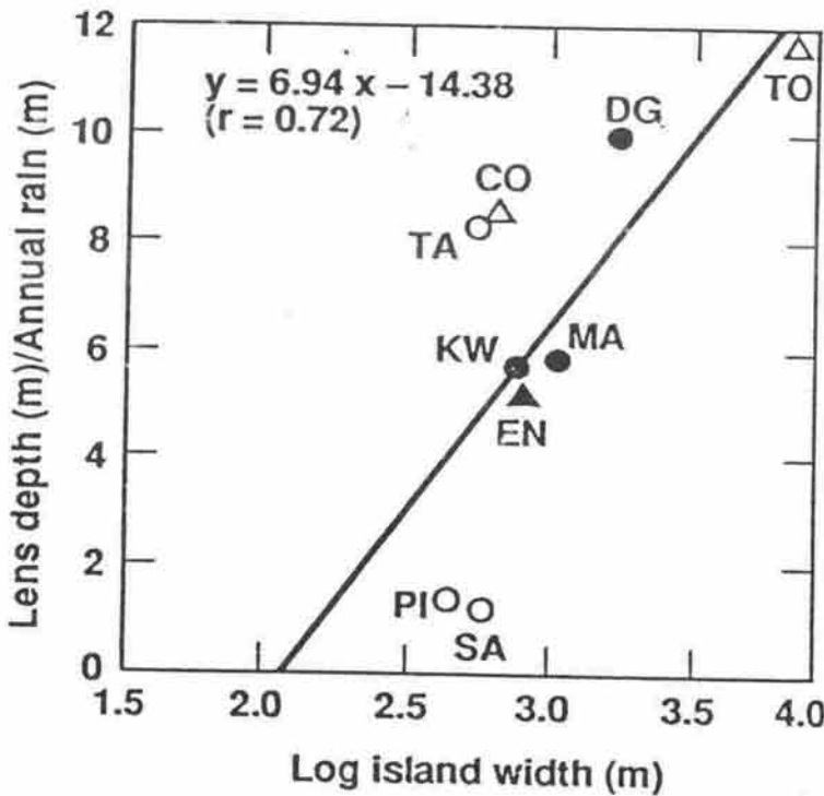
Figure 4. The ratio of fresh water lens thickness (distance from water table to 50% seawater isochlor, m) to mean annual rainfall (m) plotted against log island width (m; minimum dimension at location of freshwater lens). Island data are for Tarawa (TA; Lloyd et al. 1980), Pingelap (PI; Ayers et al. 1984), Satawan (SA; Ayers & Clayshulte 1983), Majuro (MA; Hamlin & Anthony, 1987), Kwajalein (KW; Hunt & Peterson 1980), Enjebi (EN; Buddemeier & Holladay 1977), Diego Garcia (DG; PRC Toups 1983), and Tongatapu (TO; Hunt 1979). In order of decreasing estimated reliability, lens depth data are based on salinity profiles from nested piezometers (solid circles) and open boreholes (solid diamond) or on values estimated from fresh water head (solid triangle) or surface resistivity surveys (open triangle).
