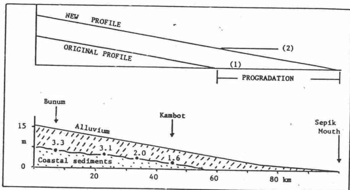
Figure 6. (a) Coastal progradation can have the same effect on river sedimentation as sea level rise. Upper diagram shows that sedimentation from original to new profile is similar to the effect of a rise from level 1 to level 2. (b) Lower diagram shows transition from coastal to alluvial sediments in lower Sepik, on transect from Bunum (locality 1 in Figure 5) to coast near Sepik mouth. Numbers on section show age of basal river deposits, in thousands of years.
