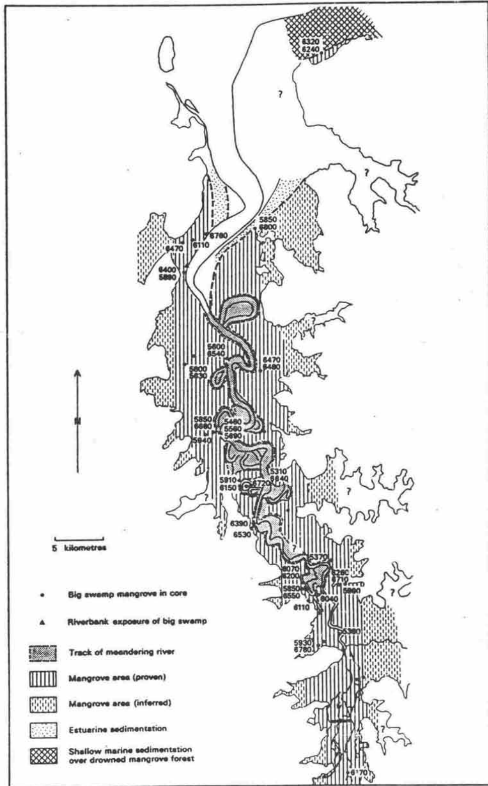
Figure 3. South Alligator tidal river and plains area, northern Australia. The map shows that part of the plains which was mangrove swamp around 6,000 years ago. Radiocarbon ages of these former mangrove swamps are shown. Today the plains, including previous meanders, are freshwater wetlands and seasonally-flooded grassland.
