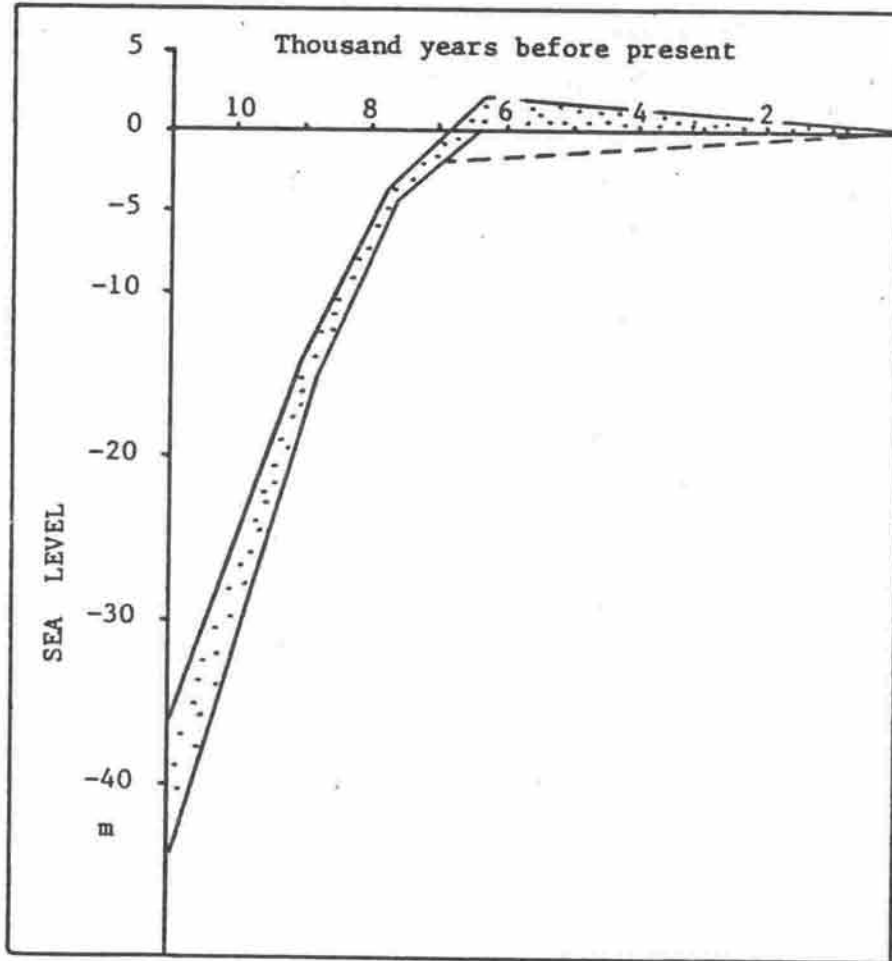
Figure 2. Sea level changes in the last 10,000 years, western Pacific region. The rise before 6,500 years ago is based on southeast Australian data (Thom & Roy, 1985). The stippled zone from 6,500 to the present covers individual curves from northern Australia and data from many Pacific islands (data in Hopley, 1987). A rising curve over the last 6,000 years (dashed line) has been identified in some other part of the world.
