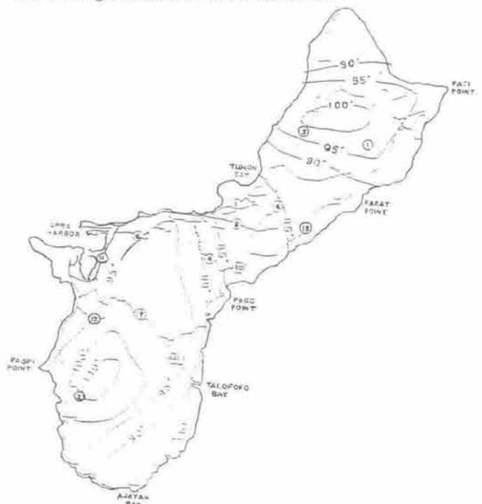
Fig. 4: Mean annual rainfall for Guam (in inches).
