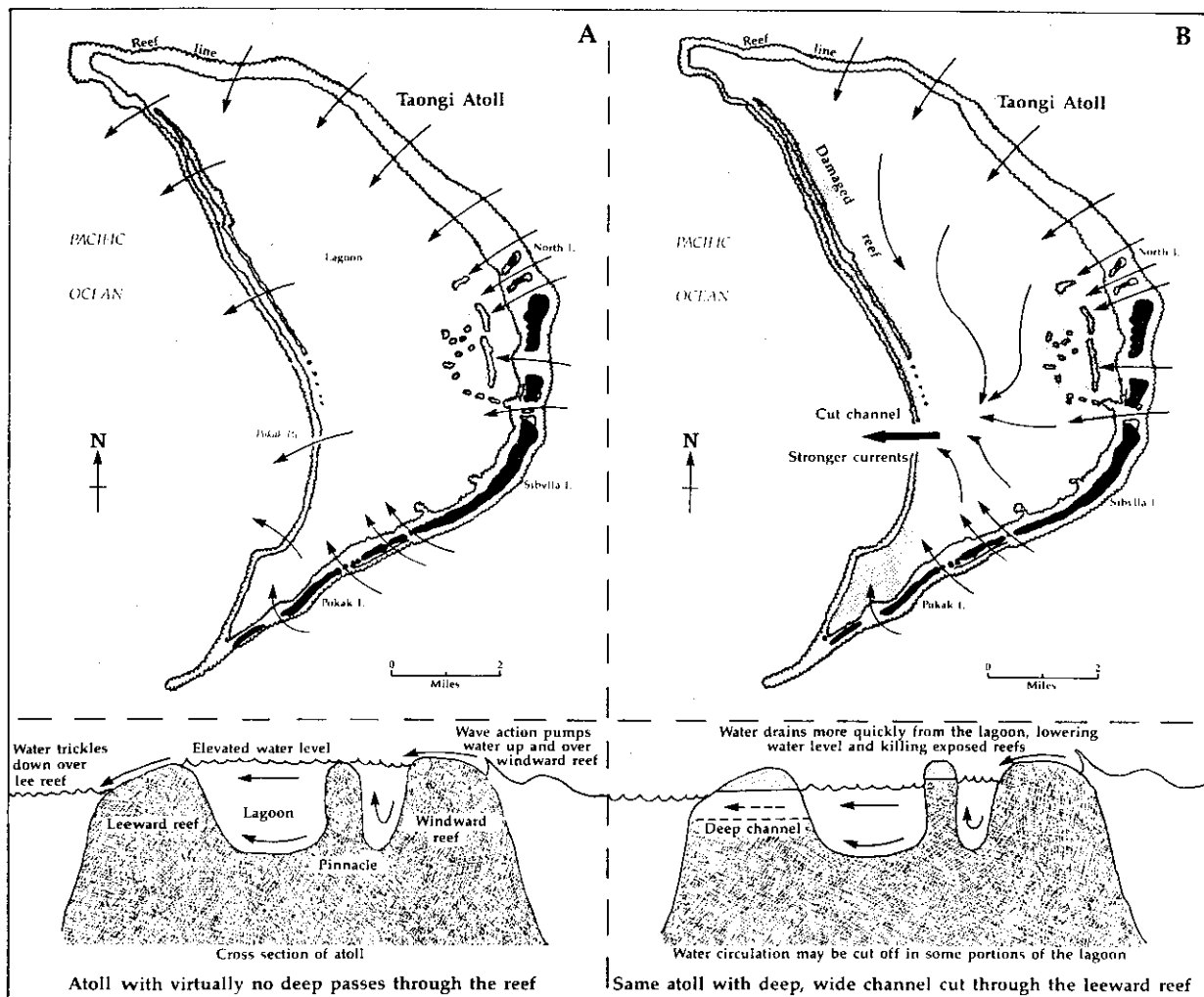
Figure IV.15. Adverse effects of cutting channels through semi-enclosed lagoons. Many atolls (including Taongi above) have elevated lagoon water levels because of wave action pumping water over windward reefs and the lack of large, deep channels to drain the excess water. The reefs grow above normal ocean sea level because of constant water flow and in response to higher lagoon water level. Cutting a deep channel through such an atoll reef would cause waters to drain more quickly, lowering lagoon water level and killing emergent reefs (After Maragos 1989).
