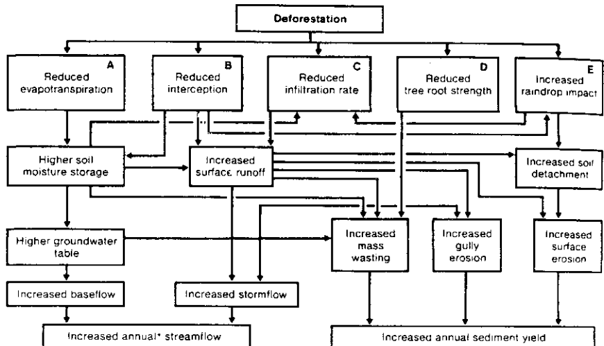
Figure V.8. Some likely hydrologic changes following deforestation (Source: Cassells et al. 1983:80. Reprinted by permission of the publisher).
