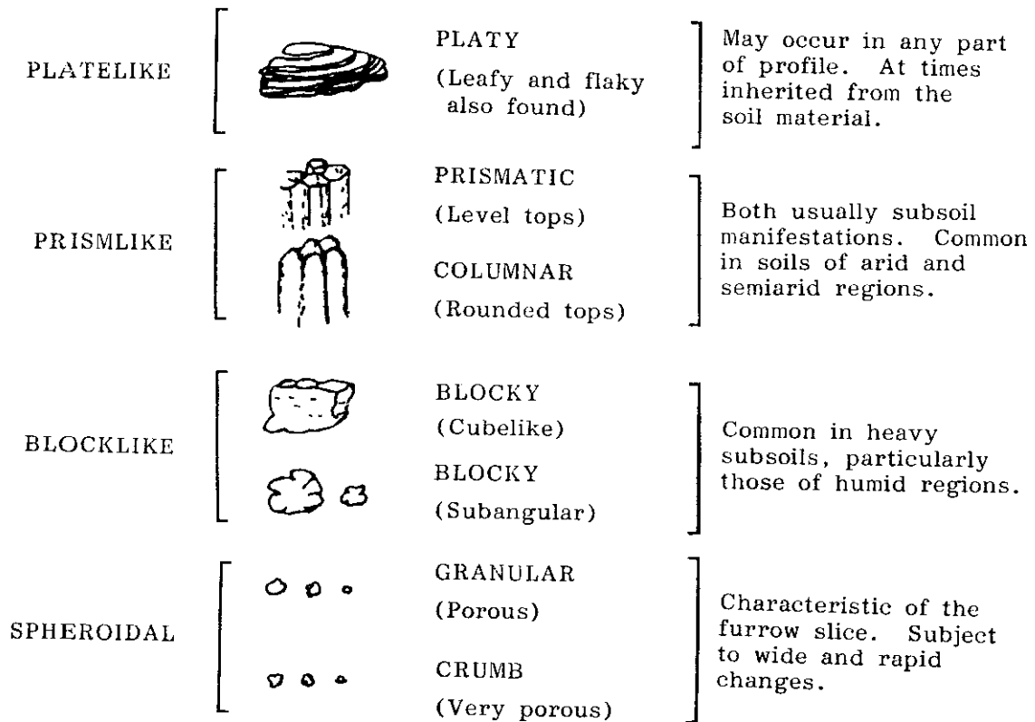
Figure V.14. Various structural types found in soils. (Reprinted with permission of Macmillan Publishing Company from The Nature and Properties of Soils , 9th ed., by Nyle C. Brady. Copyright © 1984 by Macmillan Publishing Company.)
