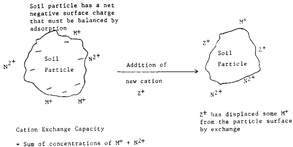
Figure V.15. Cation exchange.
