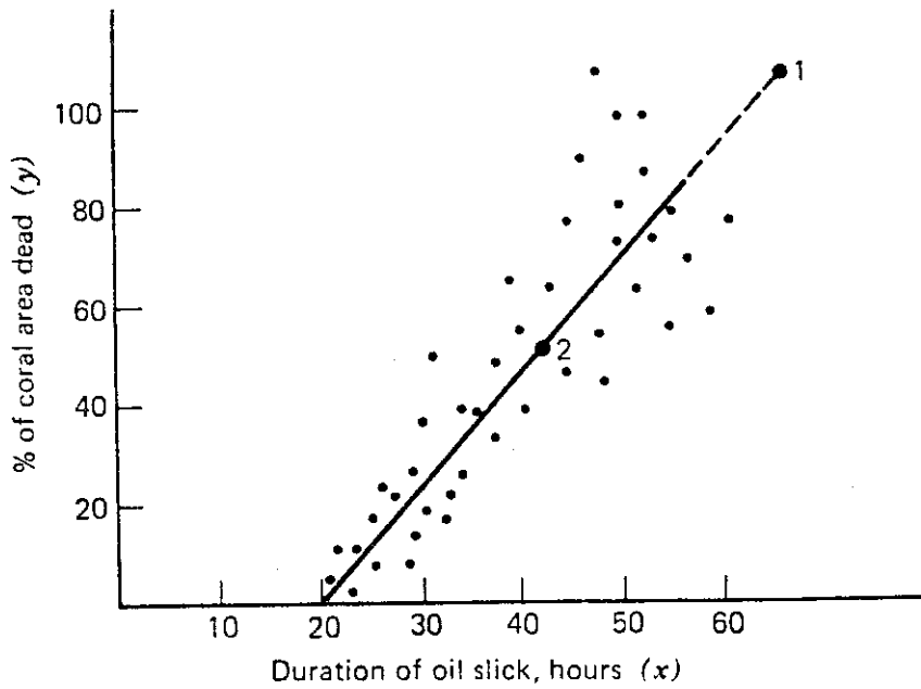
Figure II.10. Predictions by projection from past observations. The solid line is a regression line through observed events of coral death, y , under particular duration of exposure of oil, x (hypothetical data). Point 1 is predicted by extrapolation, point 2 by interpolation; both are projections from past events (Source: Ecology, Impact Assessment, and Environmental Planning , by Walter E. Westman, Copyright © 1985. Reprinted by permission of John Wiley & Sons, Inc.).
