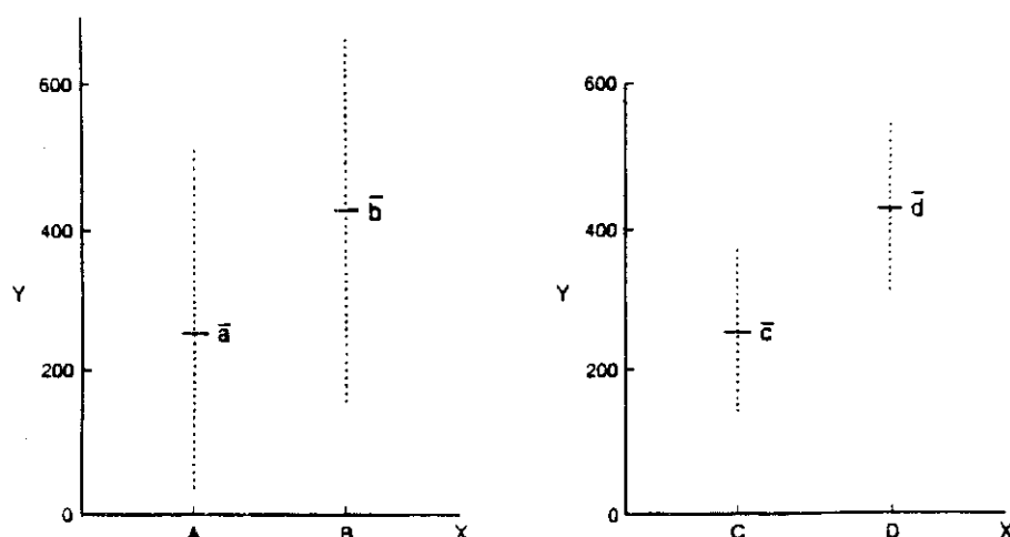
Figure III.6. Within-group and between-group variance. Assuming the same number of samples, the large variance in the populations of Groups A and B makes the difference between their means ( \bar{a} and \bar{b} ) not significant. The mean values of Groups C and D are identical to those of A and B, respectively, but the difference between \bar{c} and \bar{d} is significant because the within-group variance is small (Source: Harper et al. 1987:53).
