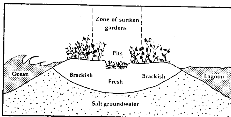
Figure III.1. Cross-section of an atoll islet with pit cultivation of babaj . The pit allows the plants access to the freshwater lens near the center of the islet. The bottomless baskets placed around the plants are filled with miscellaneous organic matter, which acts as natural fertilizers and soil conditioners and sustains yields permanently. (Adapted from Klee 1980. Reprinted by permission of the publisher.)
