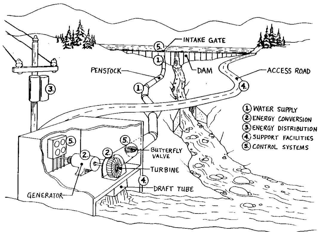
Figure IV.5. Basic elements in a hydroplant (Source: Rochester et al. 1984).
