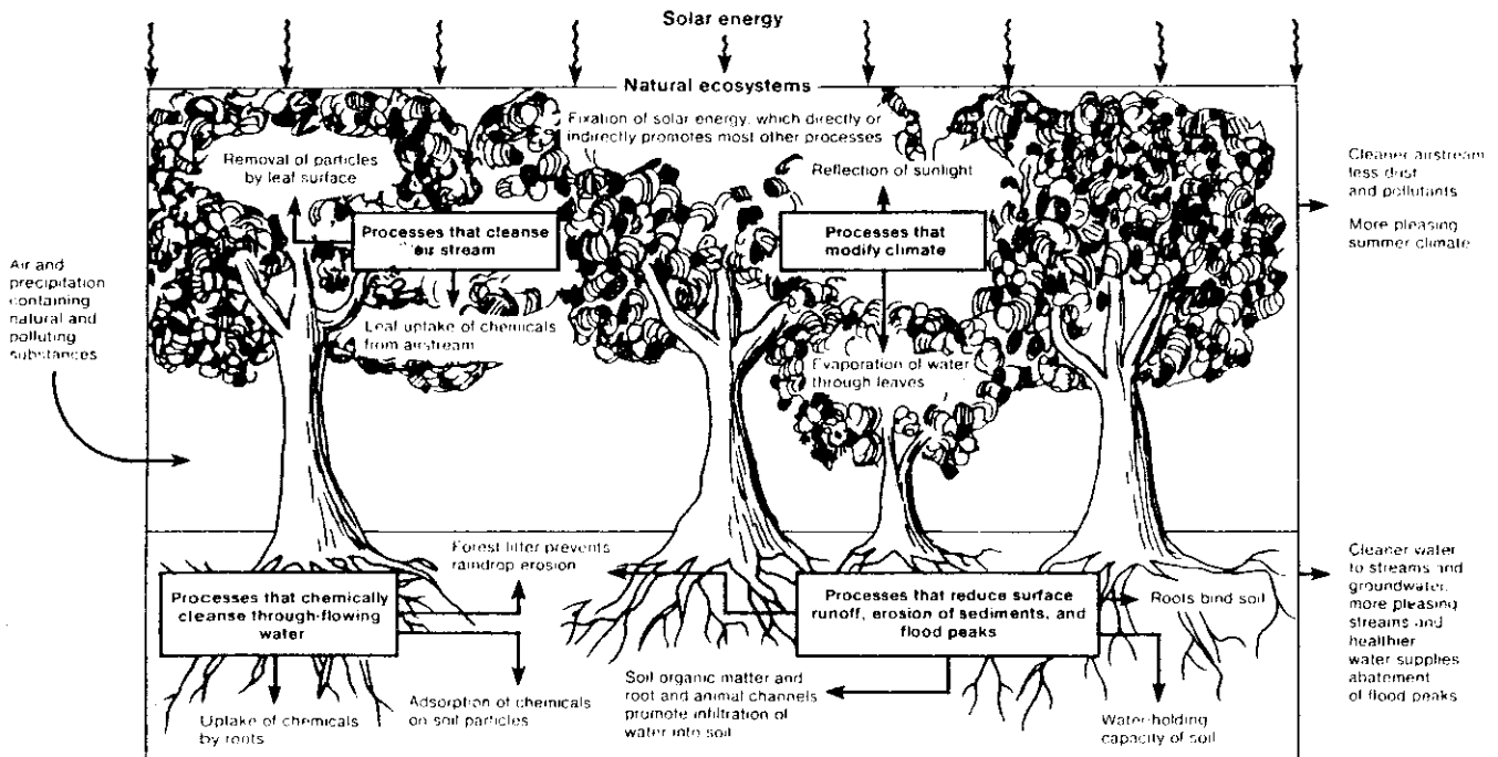
Figure V.7. Some forest ecosystem processes providing services valued by society (Source: F.H. Bormann, "An Inseparable Linkage: Conservation of Natural Ecosystems and the Conservation of Fossil Energy." Bioscience 26(12)754-760. Copyright © 1976 by the American Institute of Biological Sciences. Reprinted by permission of the publisher and the author).
