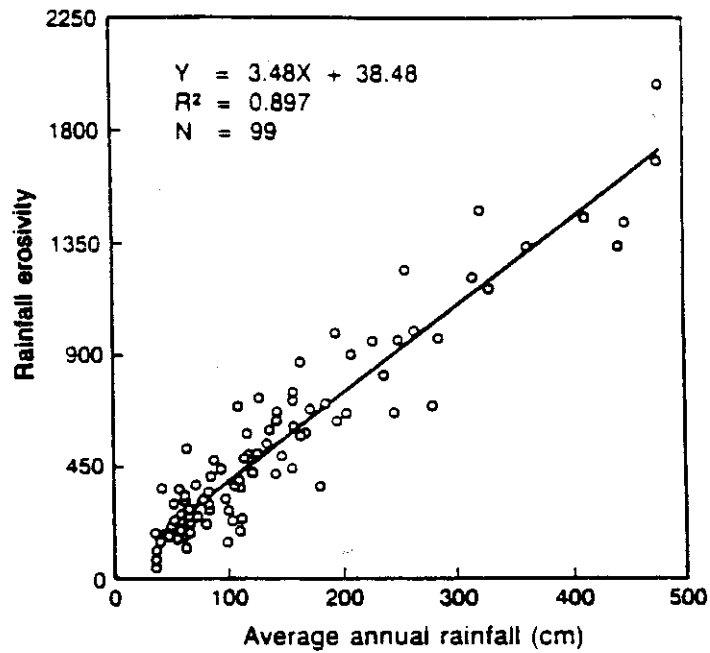
Figure III.8. Regression relationship between erosivity values and average rainfall. The regression line represents the "best fit" of the line to the data and is described by the equation Y = 3.48X + 38.48 (Source: Adapted from Lo et al. 1985:388. Reprinted with permission).
