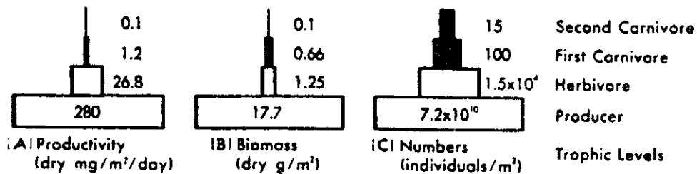
Figure V.1. Pyramids of productivity, biomass, and numbers for an experimental pond. (Reprinted with permission of Macmillan Publishing Company from Communities and Ecosystems by Robert H. Whittaker. Copyright © 1975 by Robert H. Whittaker.)
