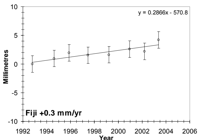
Figure 26. Movement of the SEAFRAME Sensor relative to the Tide Gauge Bench Mark.
