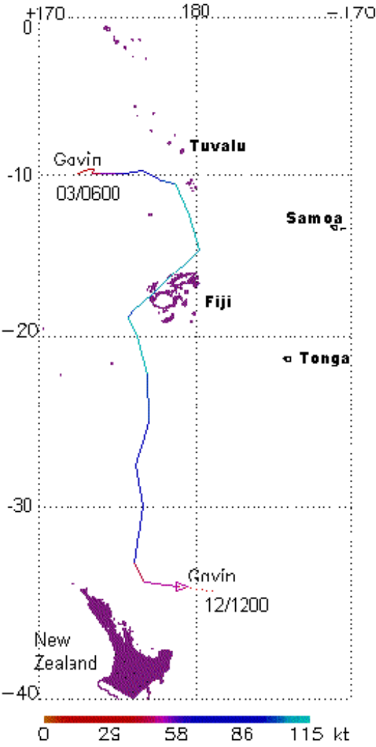
Figure 10. Track of Tropical Cyclone Gavin, March 1997
