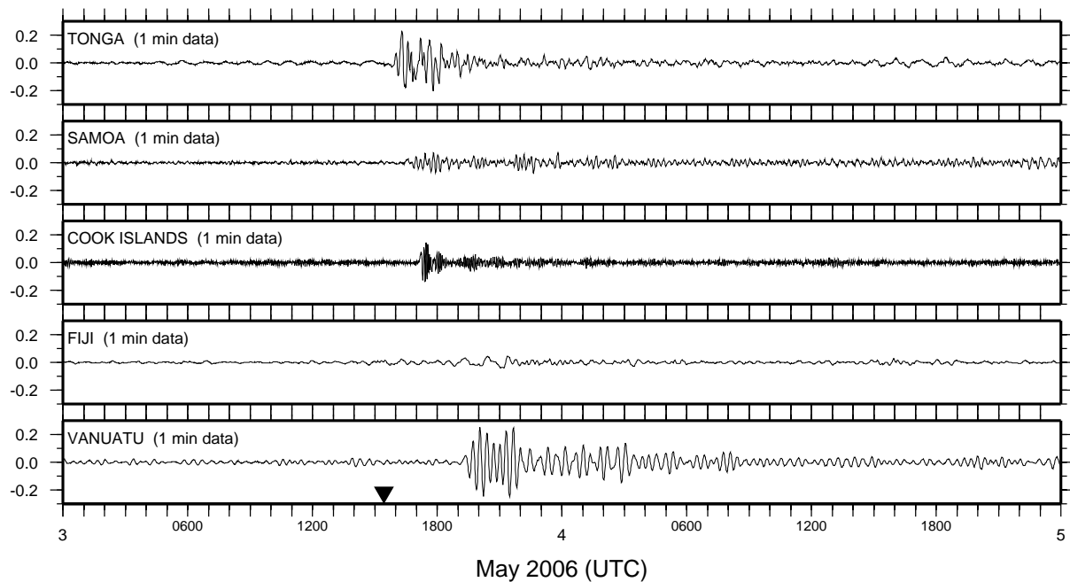
Figure 17. The non-tidal sea level record (m) at SEAFRAME stations following a tsunamigenic earthquake near Tonga at 15:27 UTC on 3 May 2006.
