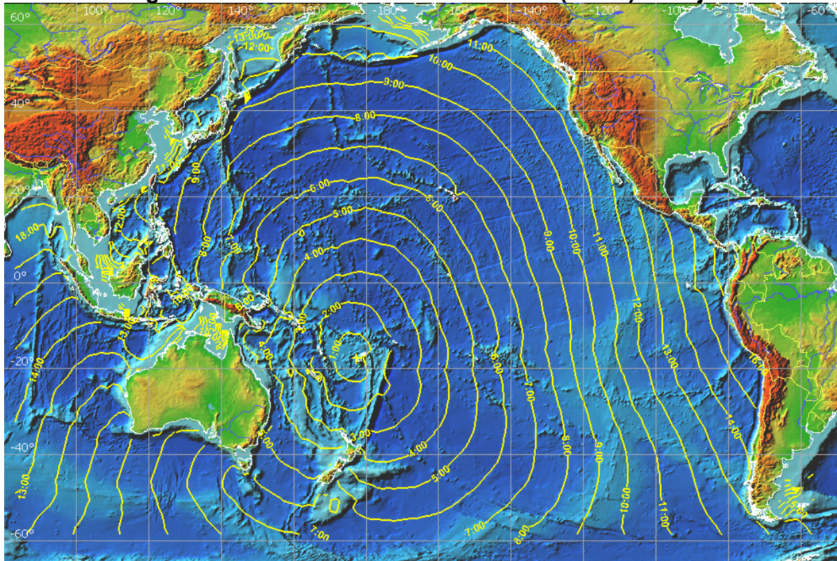
Figure 14. Inverse Tsunami Travel Times (hours) for Fiji.
