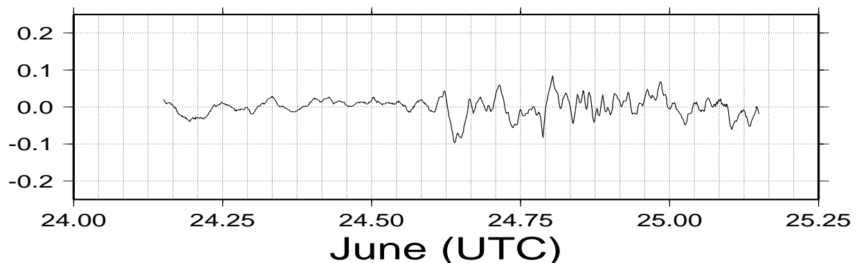
Figure 15. The non-tidal sea level record (m) at Lautoka in June 2001 following a tsunamigenic earthquake off Peru.
