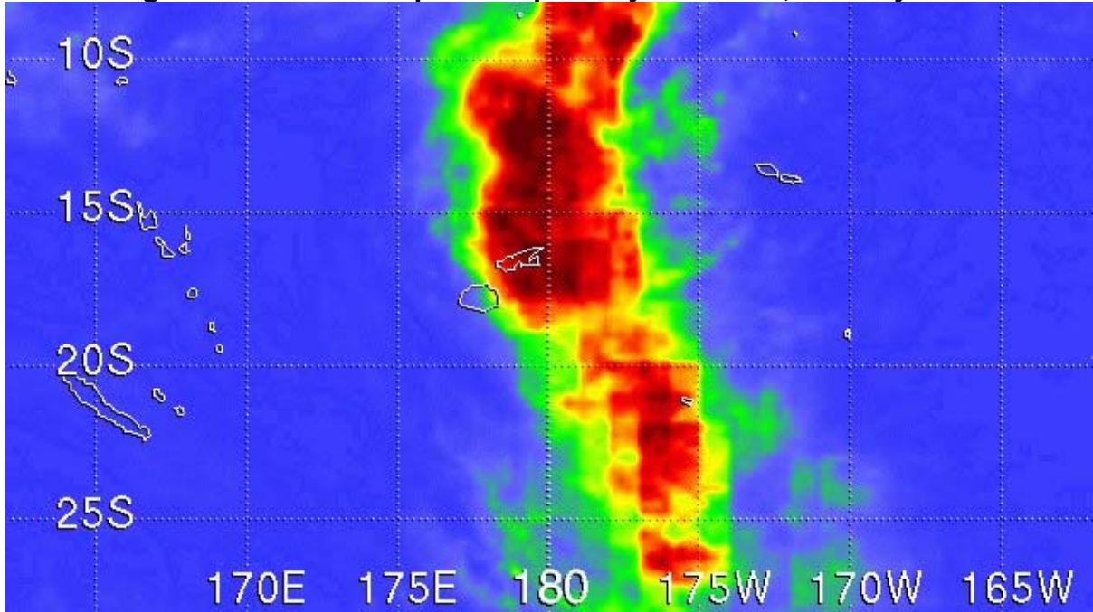
Figure 11. Rainfall Map for Tropical Cyclone Ami, January 2003
