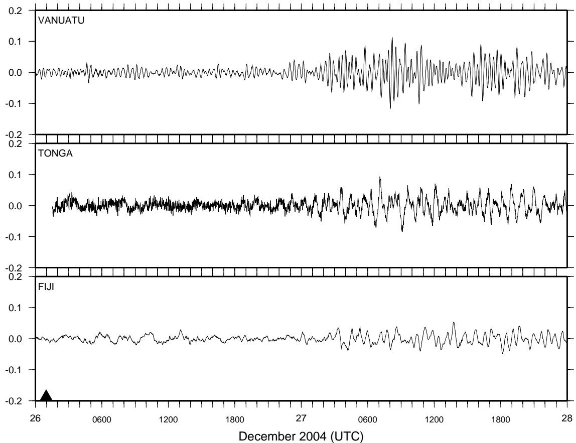
Figure 16. Non-tidal Sea Level Signal (m) following the 26 December 2004 Indian Ocean Earthquake.
