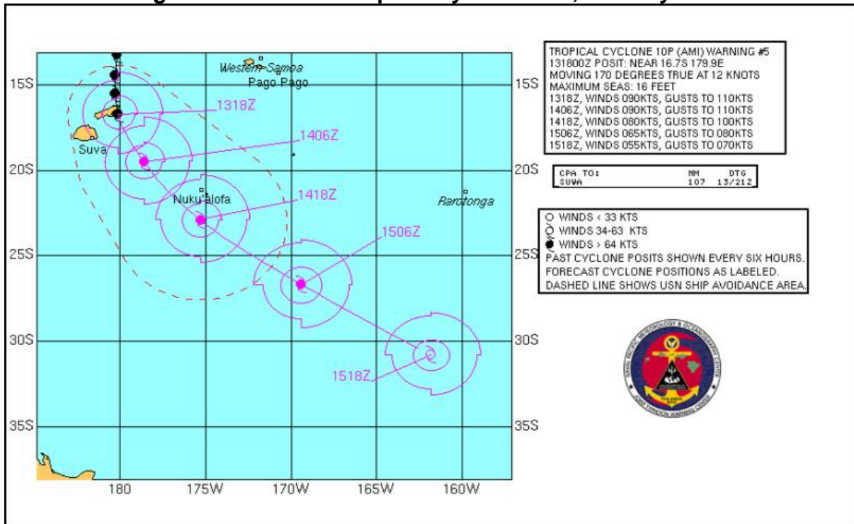
Figure 12. Track of Tropical Cyclone Ami, January 2003
