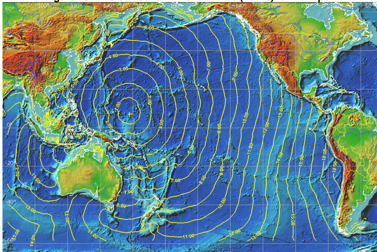
Figure 10. Inverse Tsunami Travel Times (hours) for Pohnpei.
