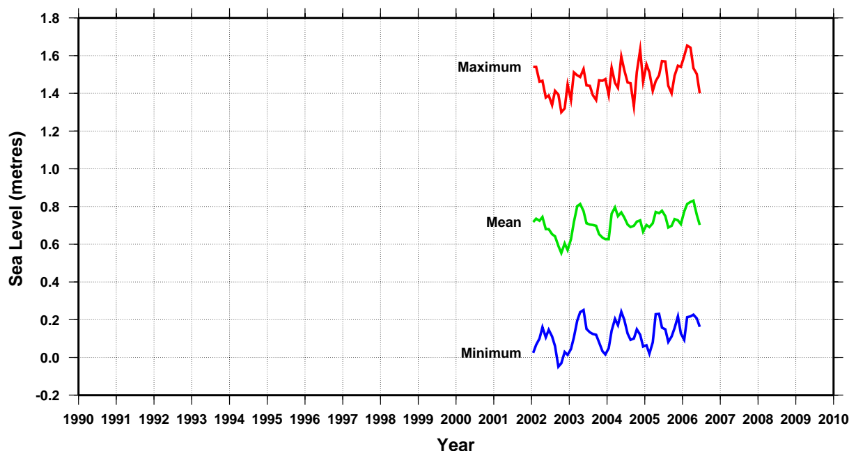
Monthly sea level at Pohnpei SEAFRAME gauge
