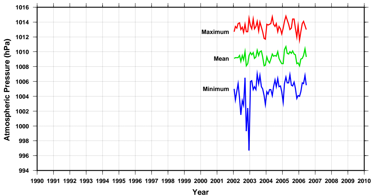
Monthly atmospheric pressure at Pohnpei SEAFRAME gauge
