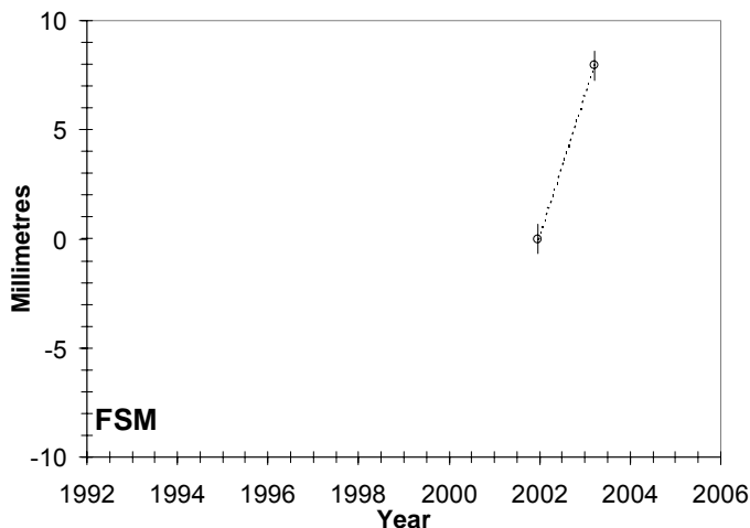
Figure 22. Movement of the SEAFRAME Sensor relative to the Tide Gauge Bench Mark.
