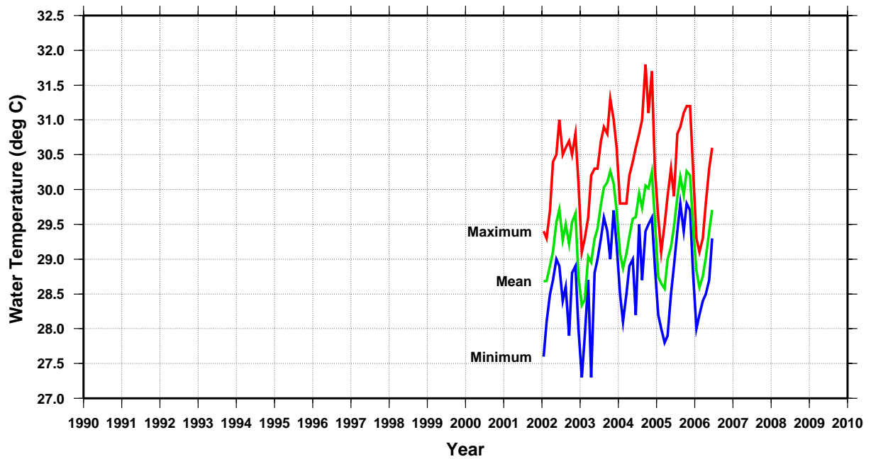
Monthly water temperature at Pohnpei SEAFRAME gauge
