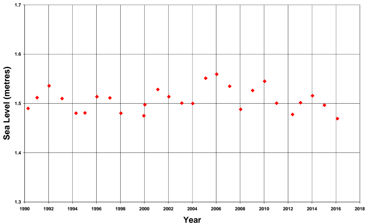
Predicted highest tide each year for Pohnpei
