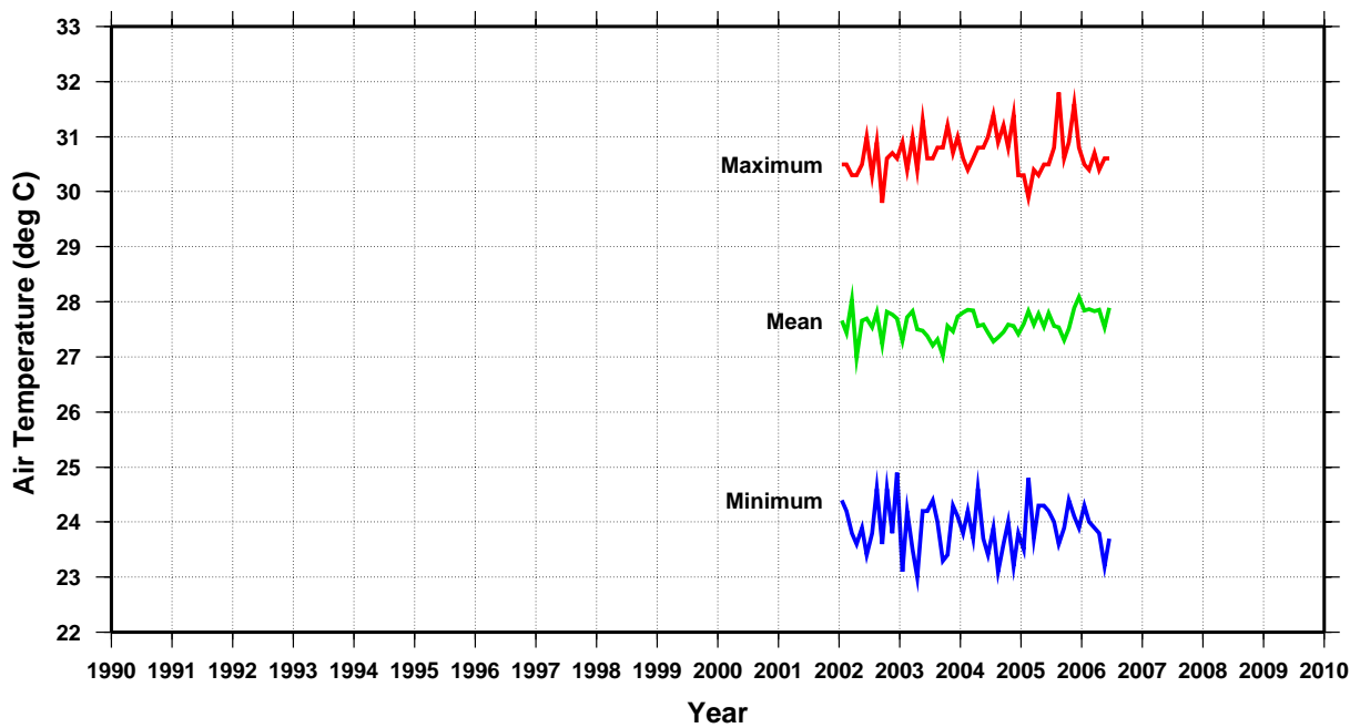
Monthly air temperature at Pohnpei SEAFRAME gauge
