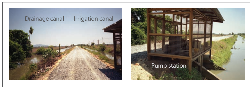
Figure 5.9 Drainage and irrigation canals and pump station for water reuse
