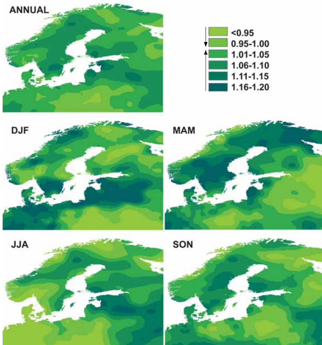
Figure 4. Annual and seasonal precipitation ratios between 1976–2000 and 1951–1975 based on VASclimO data (Beck et al., 2005) (DJF= December, January, February; MAM=March, April, May; JJA=June, July, August; SON=September, October, November).
