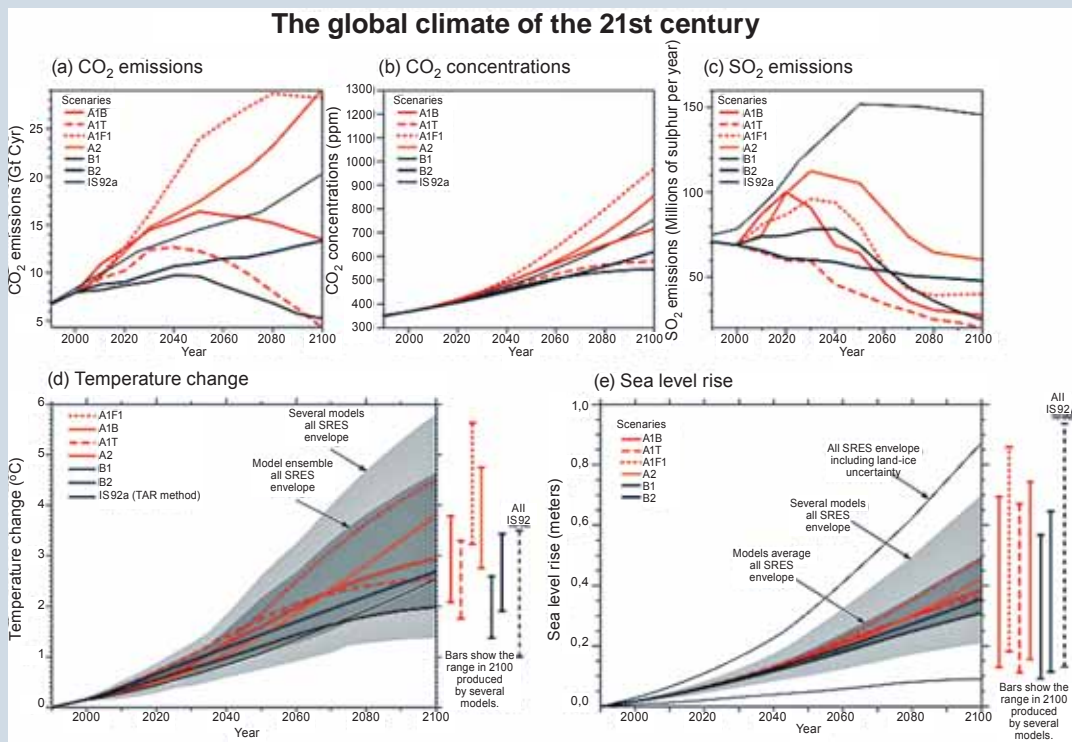
A summary of some key factors related to global climate change in the 21 st century, as presented in the IPCC Third Assessment Report (IPCC (2001), Summary for Policymakers, Figure 5), is shown here: (a) CO 2 emissions of the six illustrative SRES scenarios along with an older scenario (IS92a) used in the IPCC Second Assessment Report; (b) projected CO 2 concentrations; (c) anthropogenic SO 2 emissions (the older IS92a scenario, with very large SO 2 emissions in the late 21 st century, is now believed to be unrealistic); (d) and (e) projected global mean temperature and sea level responses, respectively. The “several models all SRES envelope” in (d) and (e) shows the temperature and sea level rise, respectively, for a simple climate model forced with all 35 SRES scenarios and tuned separately to mimic the behaviour of seven complex climate models. The “model average all SRES envelope” shows the average from these models for the range of scenarios. The diagrams do not include all sources of uncertainty.
