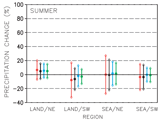
Figure 13. Seasonal GCM-derived 95% probability intervals of precipitation change in percent. Intervals are given separately for the A1FI (red), A2 (black), B2 (blue), and B1 (green) scenarios. The dot in the centre of the bar denotes the median of the interval.
