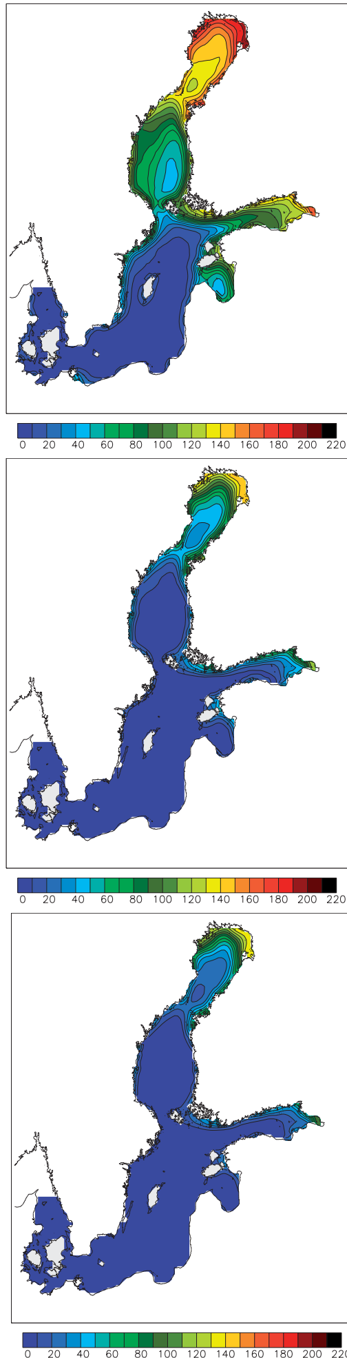
Figure 16. Mean number of ice days averaged for regional downscaling simulations of HadAM3H and ECHAM4/OPYC3: control (top panel), B2 scenario (middle panel), and A2 scenario (bottom panel). (Figure adapted from Meier et al., 2004.)
