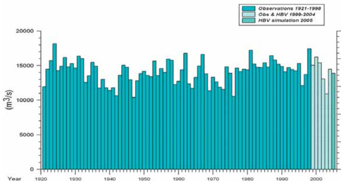
Figure 6. Total runoff to the Baltic Sea for the period 1921–2005. The period 1921–1998 is based on data from the BALTEX hydrological database. For the period 1999–2004, river flow is part of the BALTEX database and in part simulated by the HBV hydrological model (Graham, 1999). The year 2005 is entirely simulated by the HBV model.
