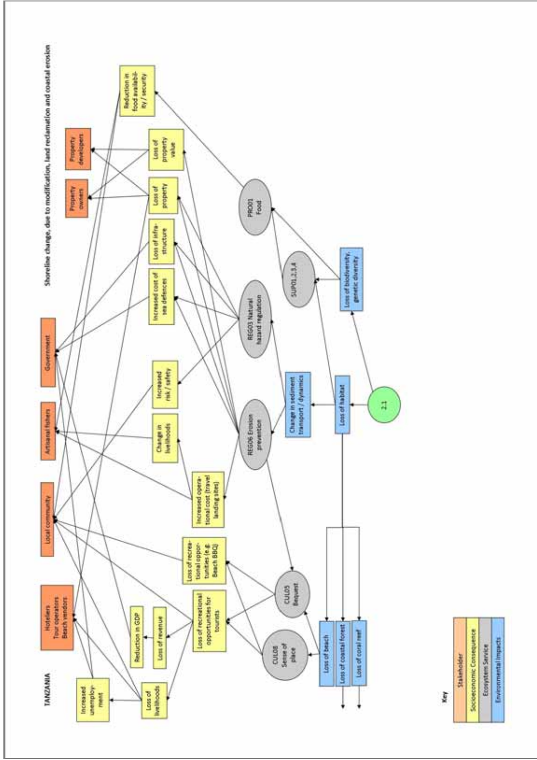
Figure 6.7.2.a: Tanzania MAC02 Impact Analysis for Issue (2.1.) Shoreline change due to modification, land reclamation and coastal erosion.
