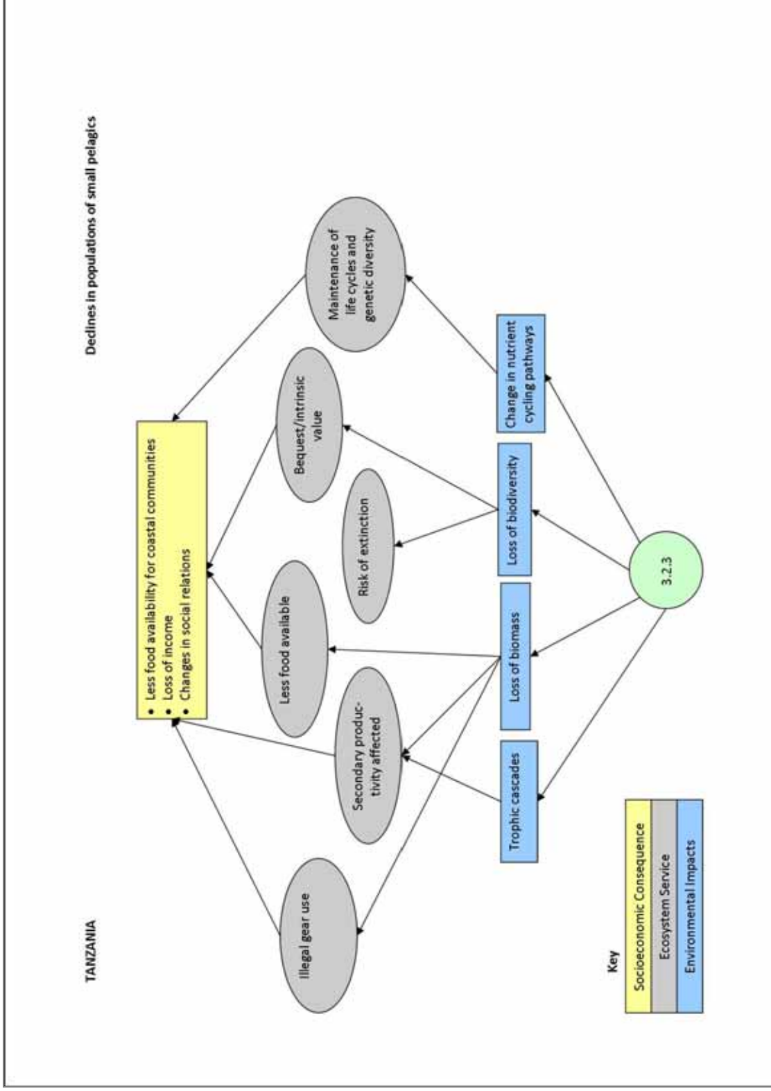
Figure 6.7.5.a: Tanzania MAC03 Impact Analysis for Issue (3.2.3.) Declines in populations of small pelagics.
