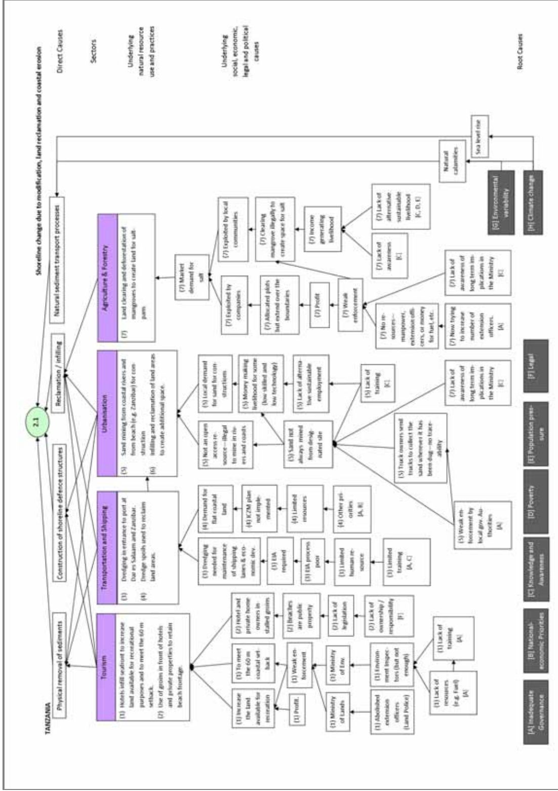
Figure 6.7.2.b: Tanzania MAC02 Causal Chain Analysis for Issue (2.1.) Shoreline change due to modification, land reclamation and coastal erosion.
