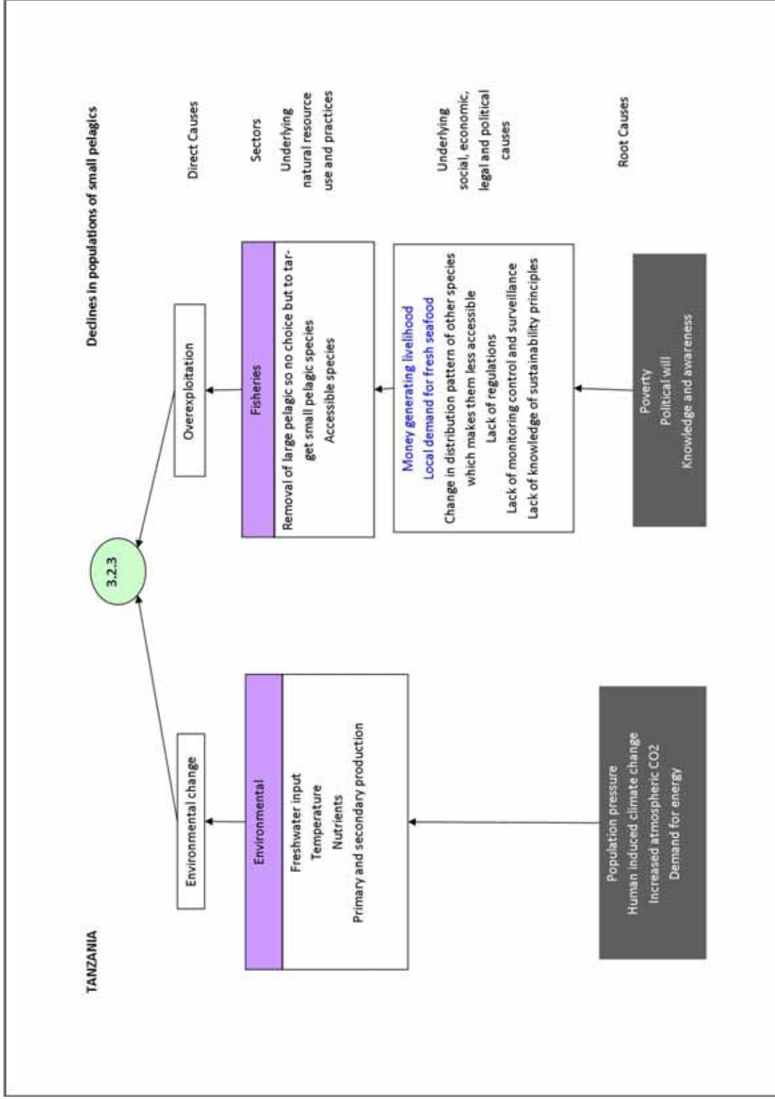
Figure 6.7.5.b: Tanzania MAC03 Causal Chain Analysis for Issue (3.2.3.) Declines in populations of small pelagics.
