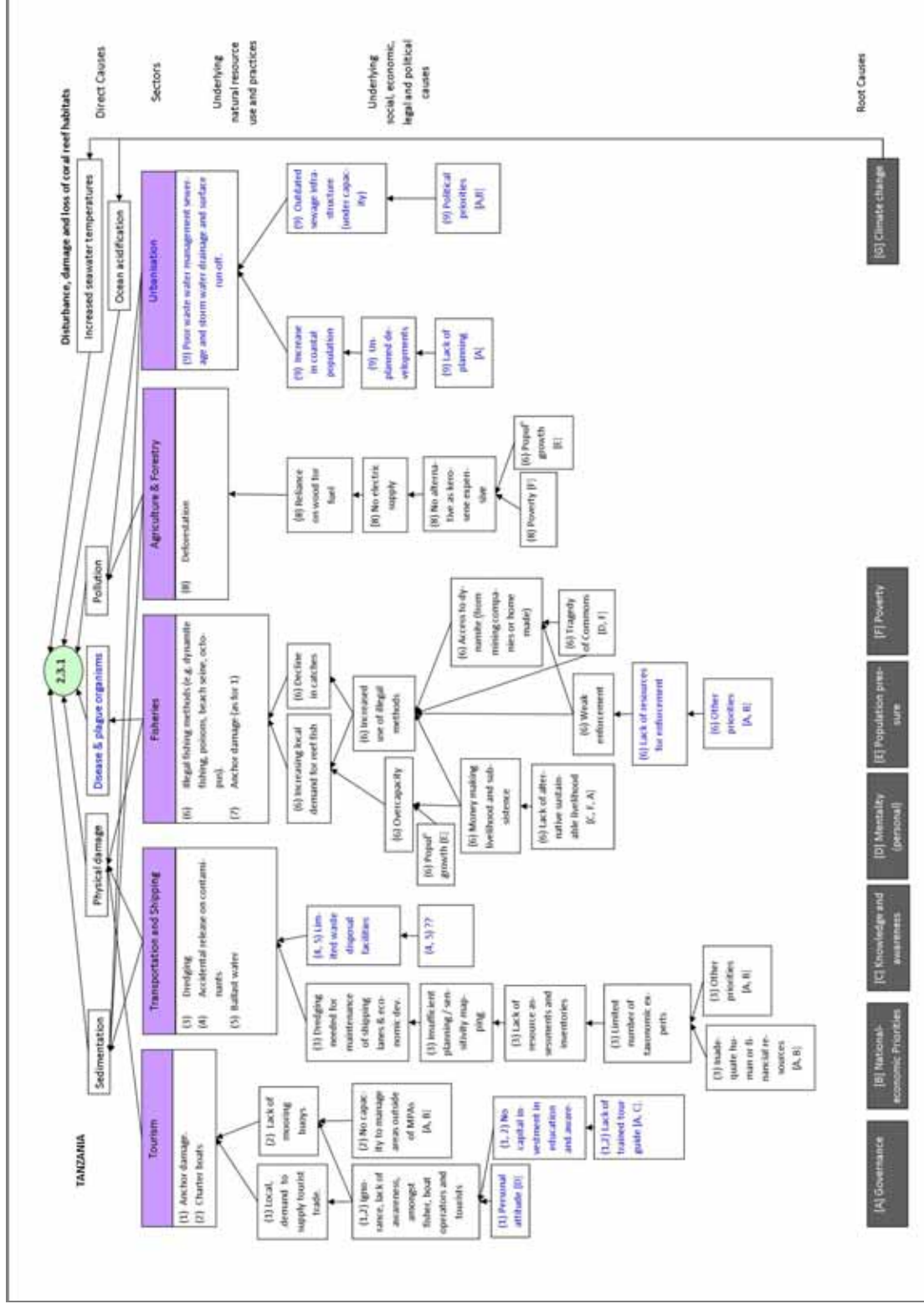
Figure 6.7.4.b: Tanzania MAC02 Causal Chain Analysis for Issue (2.3.1.) Disturbance, damage and loss of coral reefs.
