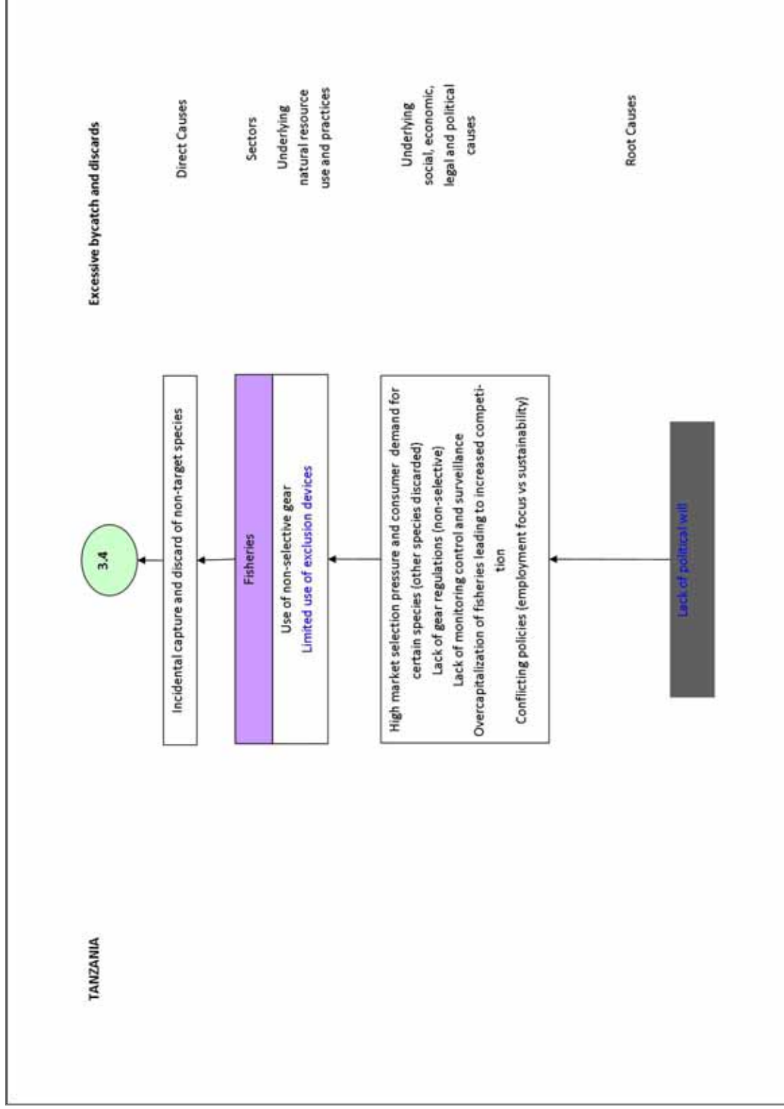
Figure 6.7.7.b: Tanzania MAC03 Causal Chain Analysis for Issue (3.4) Excessive bycatch and discards.
