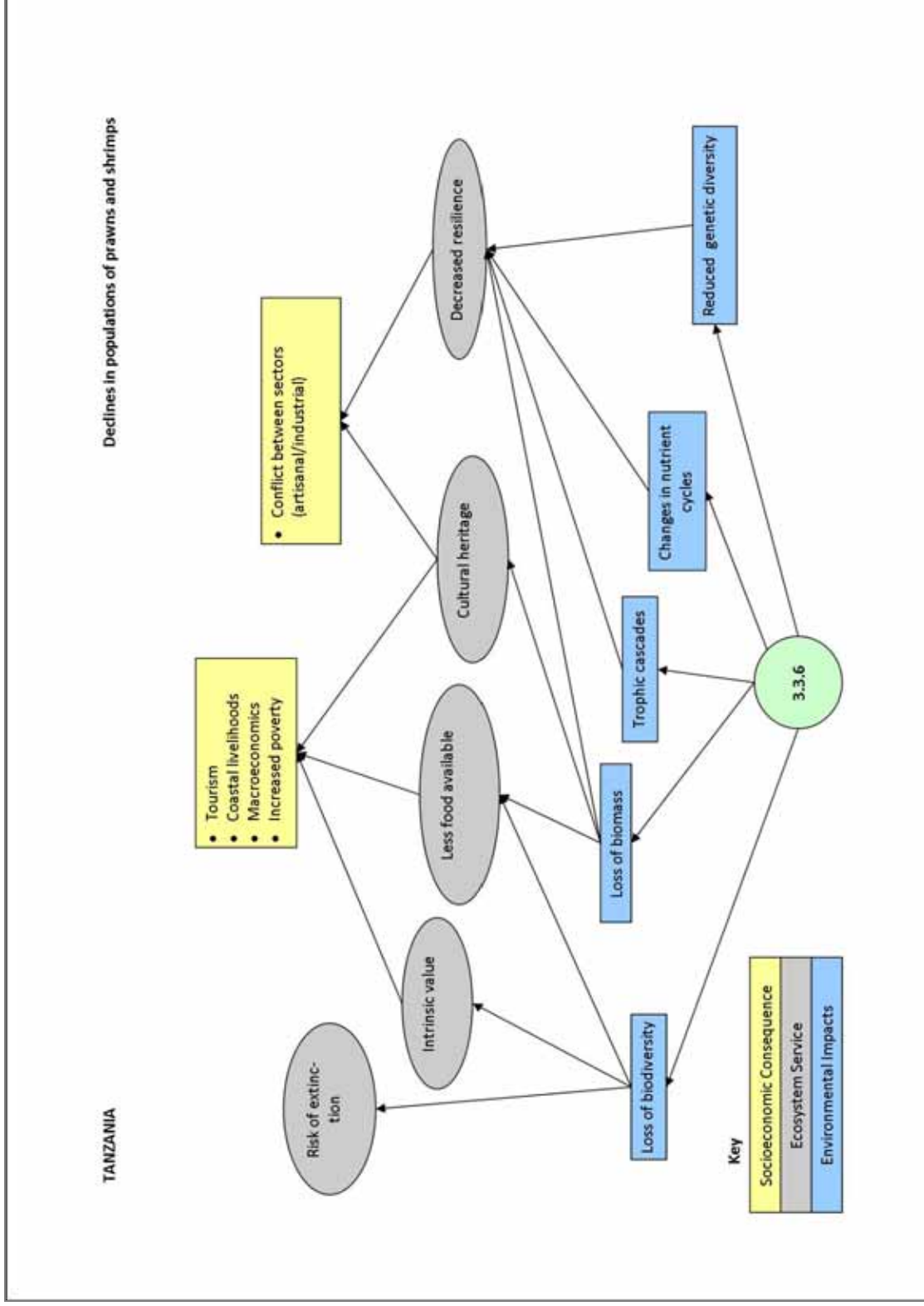
Figure 6.7.6.a: Tanzania MAC03 Impact Analysis for Issue (3.3.6.) Declines in populations of prawns and shrimps.
