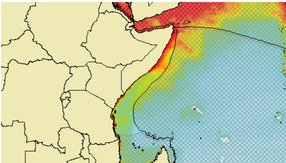
Figure 21: Mean annual primary production off the Somali coast (University of British Columbia 2007).
