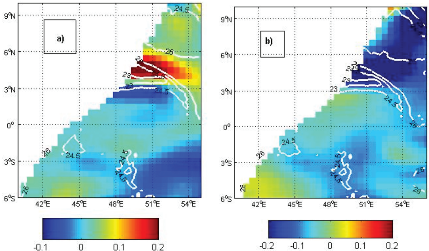
Figure 9: Maps of SST (contour in ^{\circ}\text{C} ) and a) wind stress divergence ( \text{Nm}^{-2}[104\text{km}]^{-1} ), b) wind stress curl ( \text{Nm}^{-2}[104\text{km}]^{-1} ) over the upwelling tongue during the week ending 23 July 2005. The SSTs are in contour interval of 1^{\circ}\text{C} (Adapted from Mafimbo and Reason 2010)
