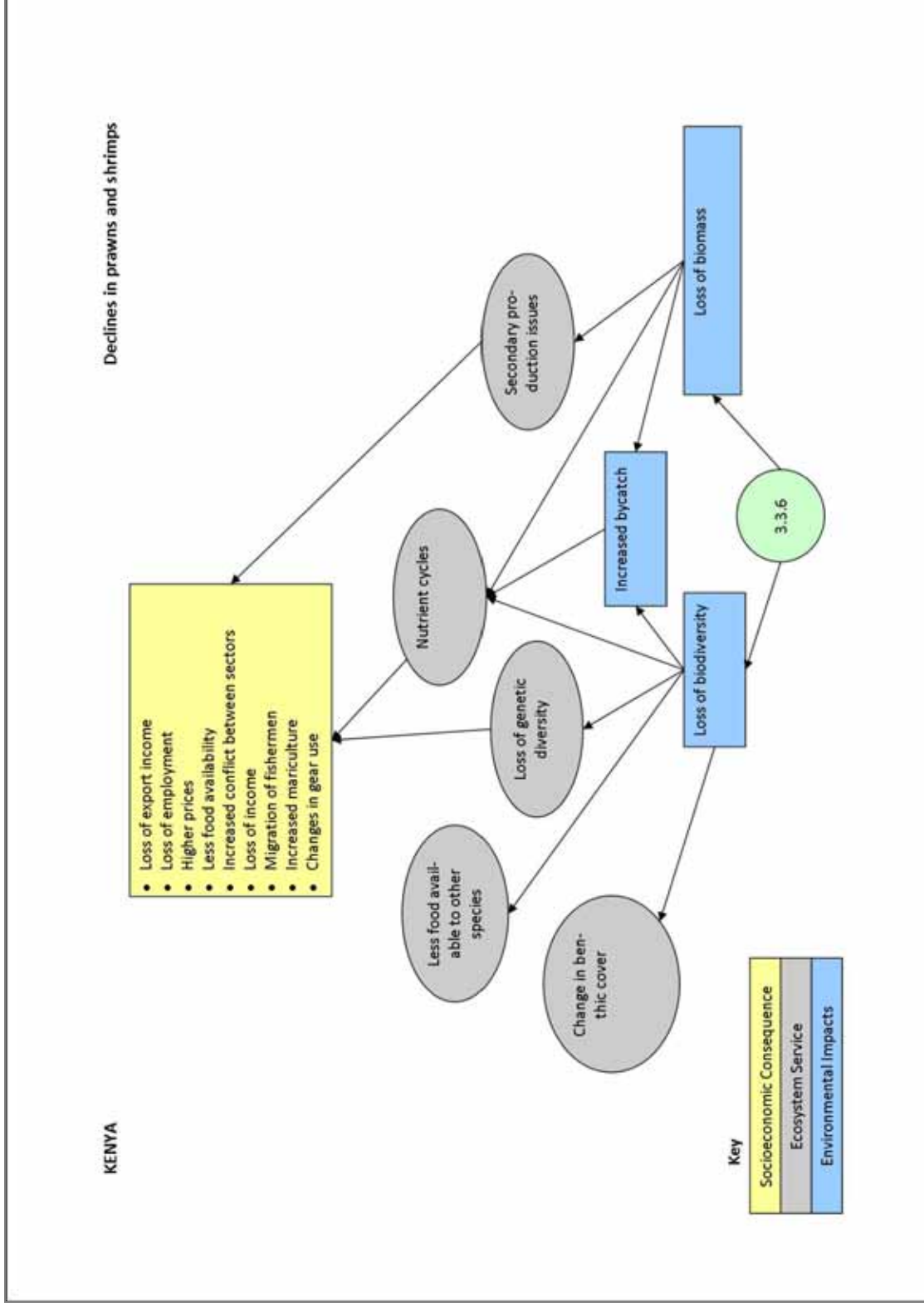
Figure 6.4.7.a: Kenya MAC03 Impact Analysis for Issue (3.3.6) Declines in populations of prawns and shrimps.
