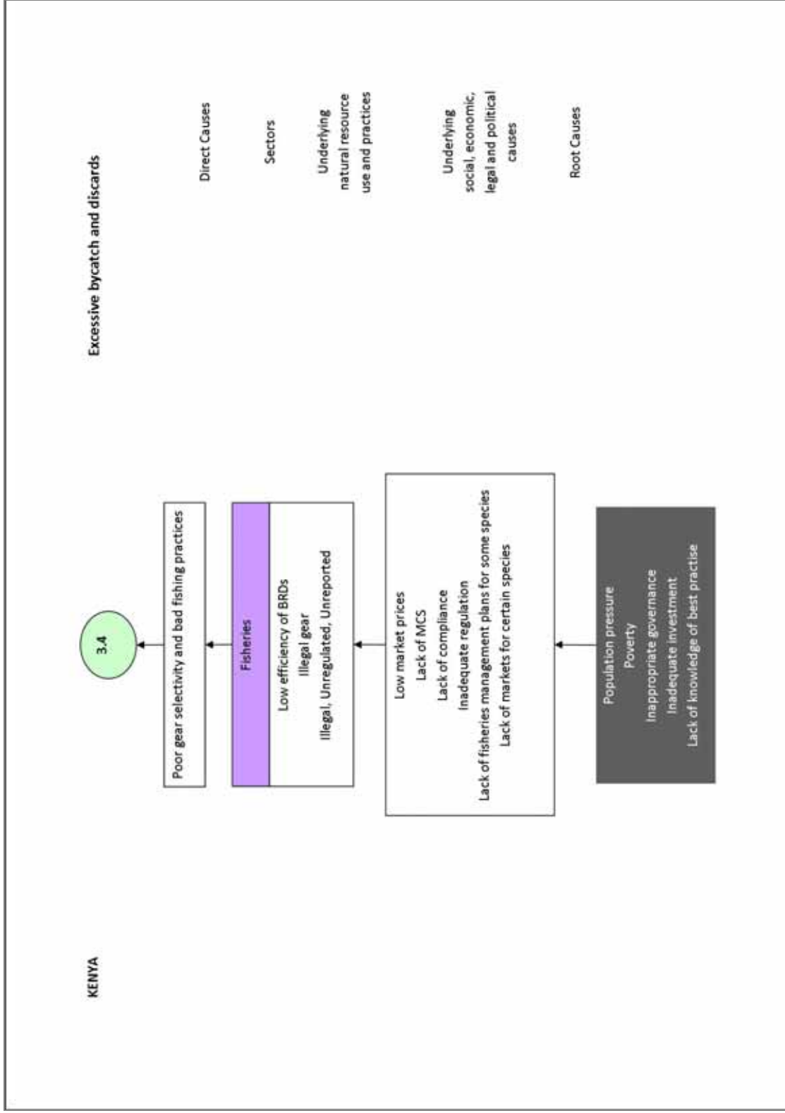
Figure 6.4.8.b: Kenya MAC03 Causal Chain Analysis for Issue (3.4) Excessive bycatch and discards.
