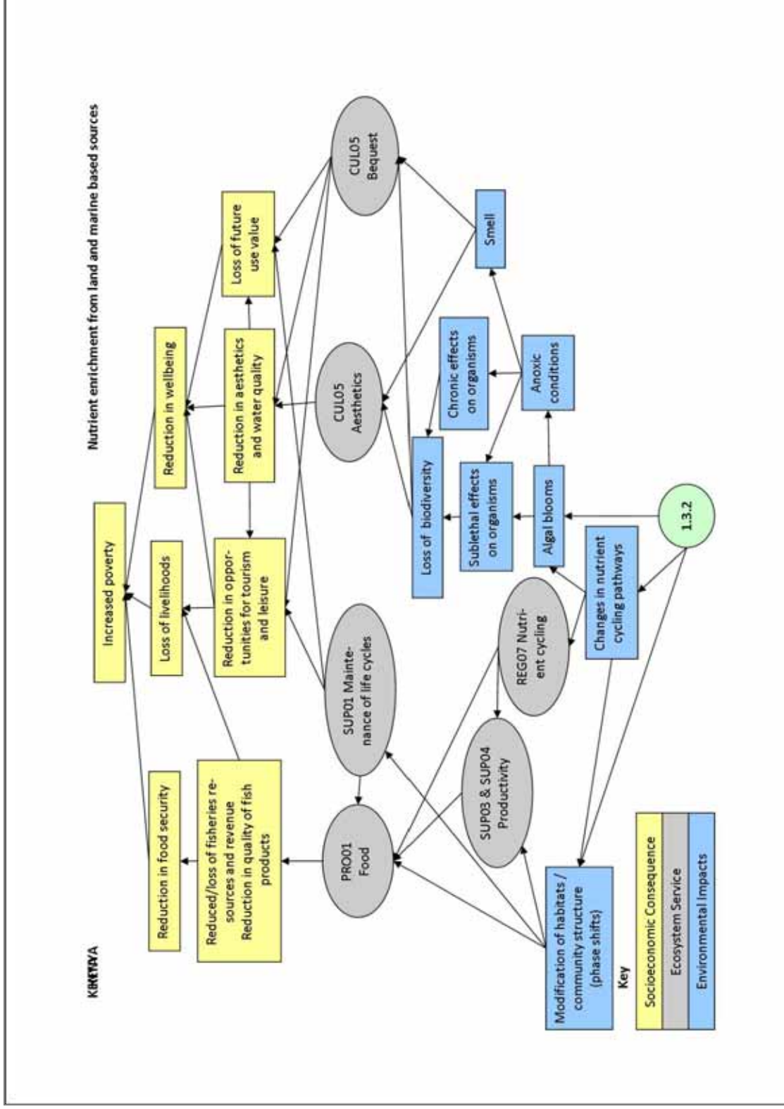
Figure 6.4.2.a: Kenya MAC01 Impact Analysis for Issue (1.3.2) Nutrient enrichment from land-based and marine sources.
