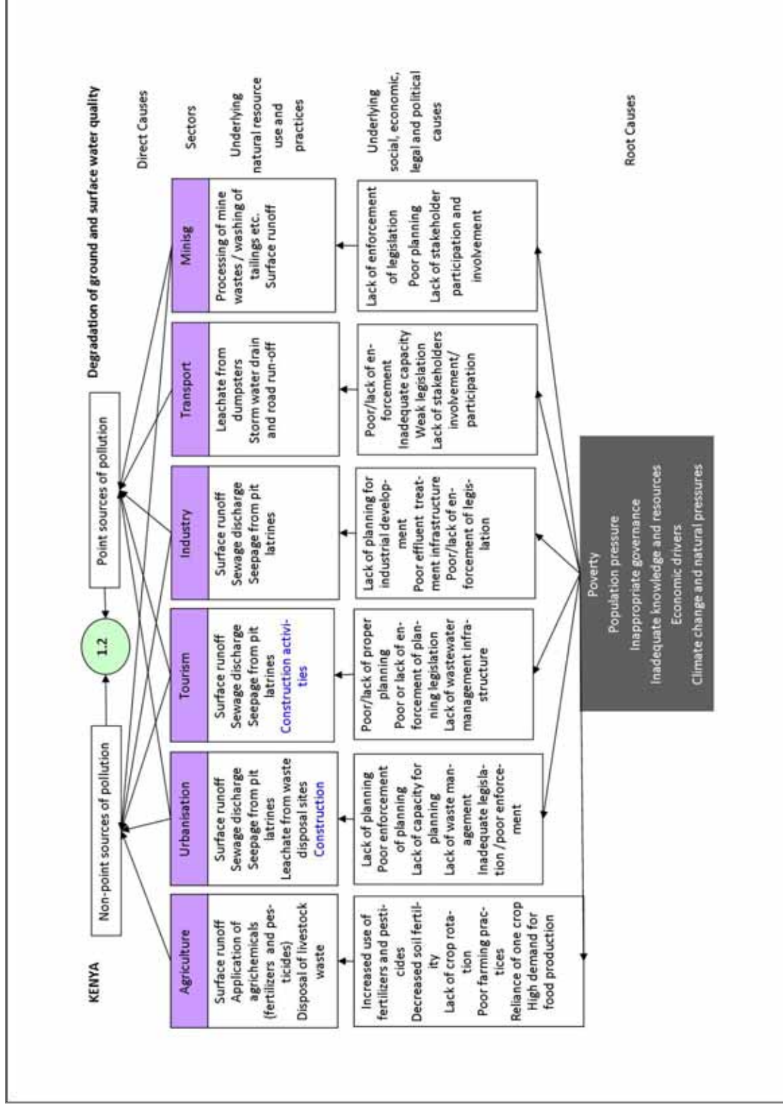
Figure 6.4.1.b: Kenya MAC01 Causal Chain Analysis for Issue (1.2) Degradation of surface and ground water quality.
