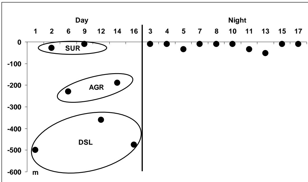
Figure 3.7.5b Depth of the different trawls performed during the Nansen cruise from 28 November to 17 December 2008. (SUR: Surface, AGR: aggregations, DSL: Deep Scattering Layer).
