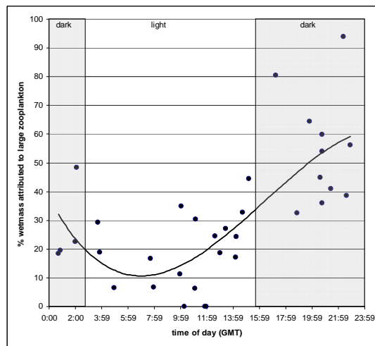
Fig. 3.7.3.1a: Percentage of total wet-mass attributed to large zooplankton (>2mm). Larger zooplankton is relatively more abundant during night stations, indicating an upward migration of larger size-classes into the top 200m during dark hours and a downward migration during day-time hours.
