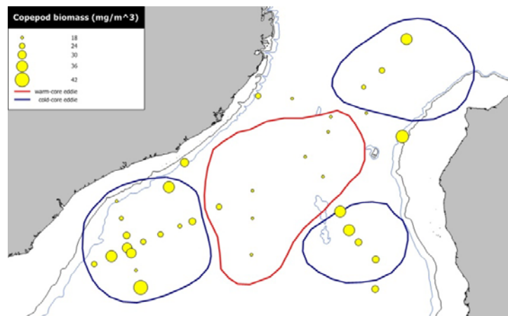
Fig. 3.7.3.1b: small copepod (<1mm) biomass distribution
