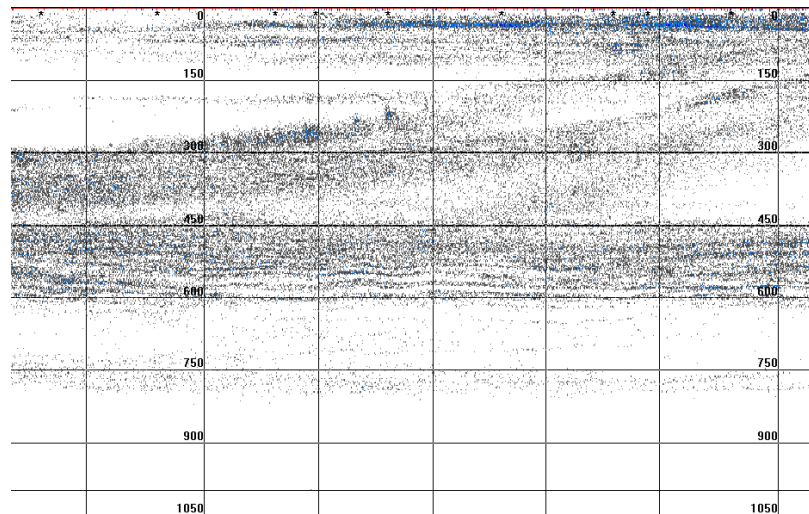
Figure 3.7.4e the rising of the DSL at dusk
