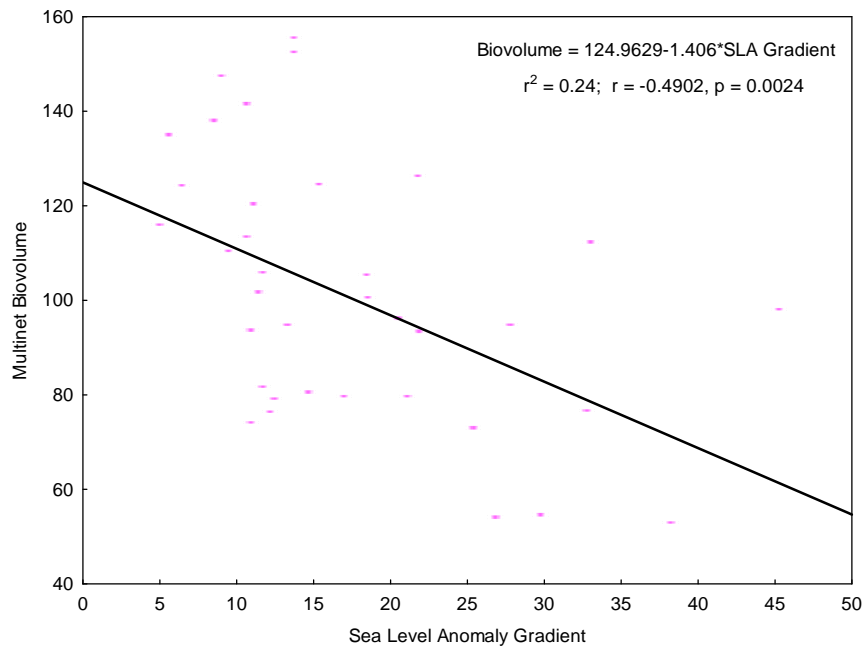
Figure 3.7.3.2e: Linear regression of Sea Level Anomaly Gradient and Multinet Biovolume ( ml.m^{-2} ) showing significant negative relationship between these variables.
