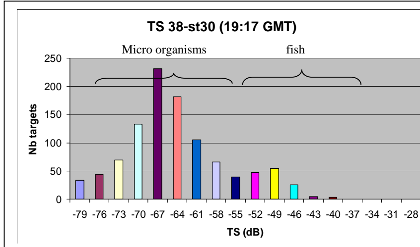
Figure 3.7.4h TS histograms with the 2 modes showing different acoustic (TS) response for fish and micro organisms (colour is only for visual discrimination purpose).
