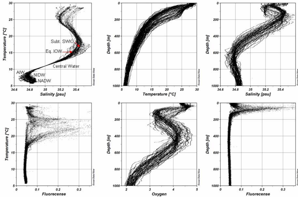
Figur 3.1.1 Stations showing TS- and TF diagrams upper and lower left.
