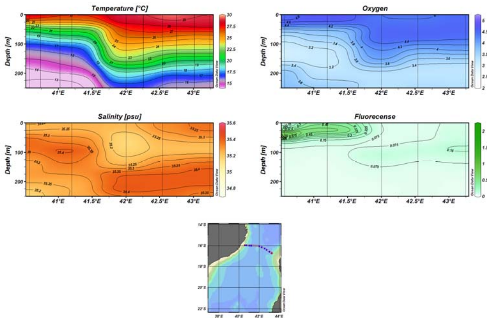
Fig.3.5.1 Vertical section in the frontal zone of a) Temperature, b) Salinity, c) Oxygen and d) Fluorescence
