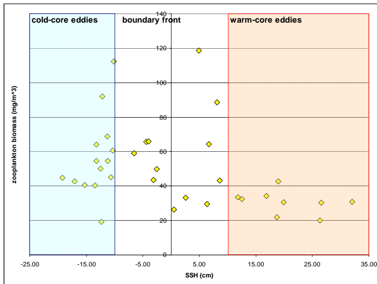
Fig.3.7.3.1d: Biomass distribution of small zooplankton (< 2mm) in relation to physical anomalies (SSH = Sea Surface Height, AVISO data).
