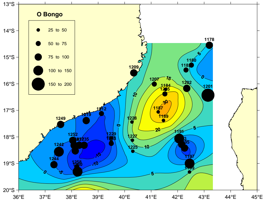
Figure 3.7.3.2c: Map of integrated macrozooplankton biovolume ( \text{ml.m}^{-2} ) from the oblique bongo in the upper 200 m at each station superimposed on a contour plot of real time sea level anomaly (SLA, cm).
