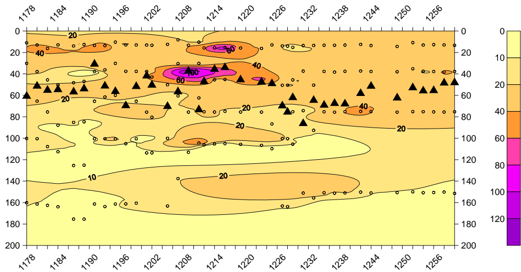
Figure 3.7.3.2a: Contour plot representing the vertical distribution of mesozooplankton biovolume ( \text{ml.m}^{-2} ) from the Multinet during the eddy study. Each data point represents the integrated biovolume from the depth stratum sampled; small circles indicate the mid-point of each depth stratum. Large triangles indicate the weighted mean depth (WMD, m) of plankton biovolume at each station. Station numbers are shown on both upper and lower X-axes.
