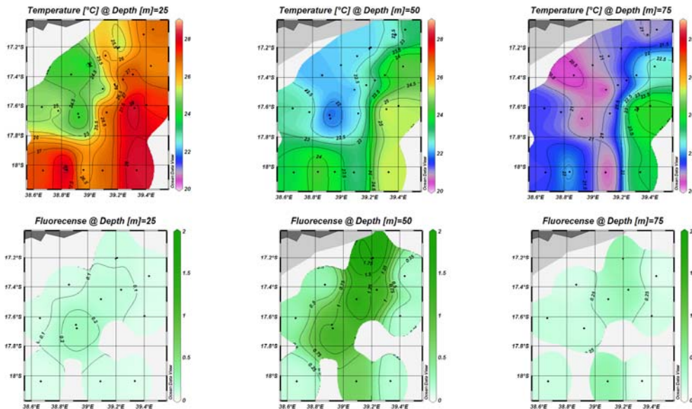
Figur 3.6.1 Horizontal distribution of temperature and fluorecence in convergence zone at 25m depth, 50m depth and 75m depth, respectively.
