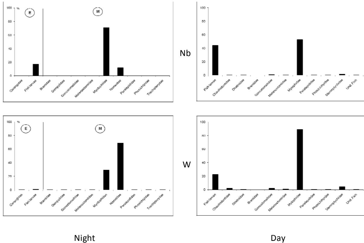
Figure 3.7.5h Repartition in number and weight (expressed in percent) of the fish catch during the Nansen cruise (28 November-17 December 2008). E = epipelagic, M = mesopeagic
