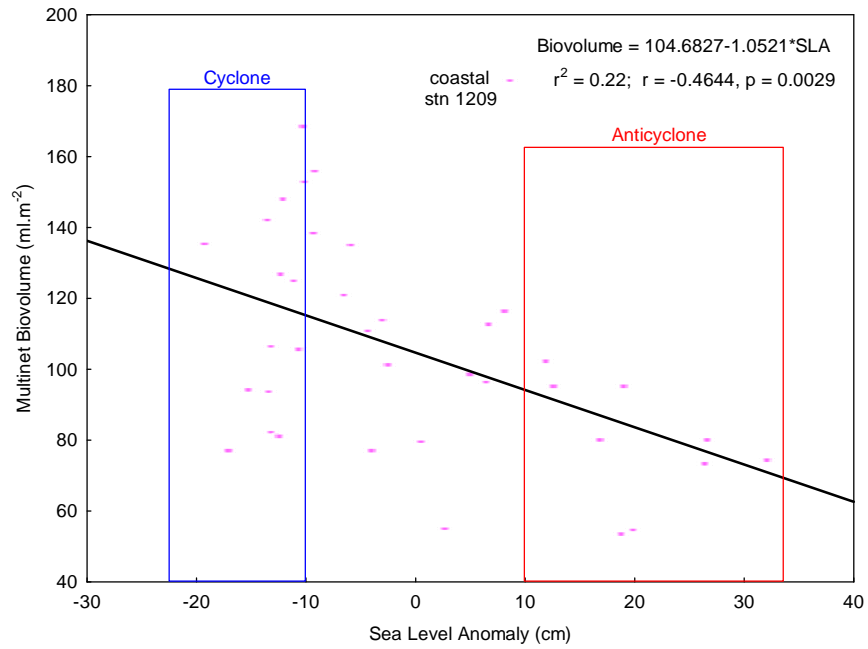
Figure 3.7.3.2d: Linear regression of Sea Level Anomaly (cm) and Multinet Biovolume ( ml.m^{-2} ) showing significant negative relationship between these variables.
