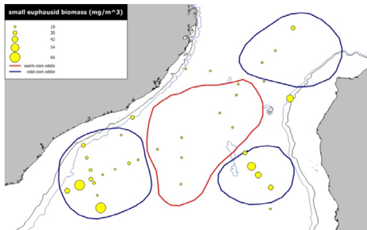
Fig 3.7.3.1c: small euphausiid (<2mm) biomass distribution
