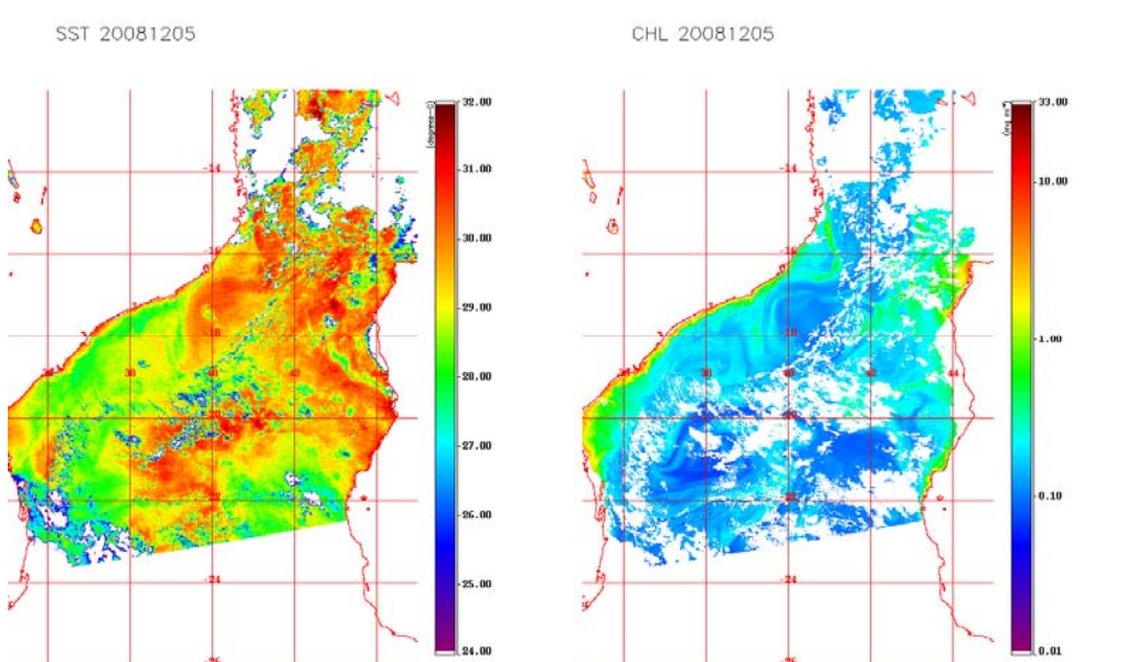
Fig.3.5.2 Chlorophyll mapping from satellite imagery obtained December 5 th 2008
