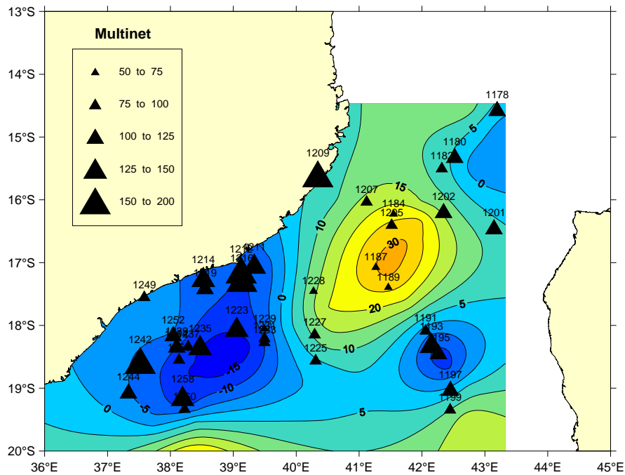
Figure 3.7.3.2b: Map of integrated mesozooplankton biovolume ( \text{ml.m}^{-2} ) in the upper 200 m at each station superimposed on a contour plot of real time sea level anomaly (SLA, cm).
