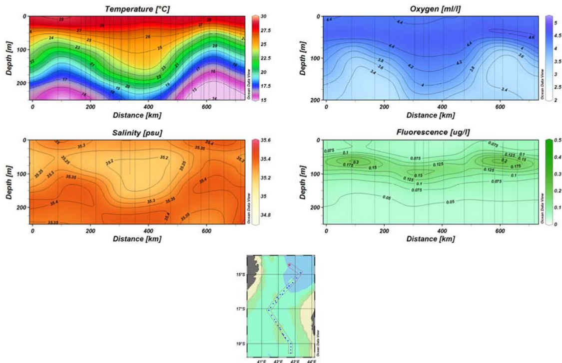
Figure 3.2.3: Vertical cross section of temperature (top left), salinity (bottom left), oxygen (top right) and fluorescence (bottom right) for the upper 250 m of the north-south transect.
