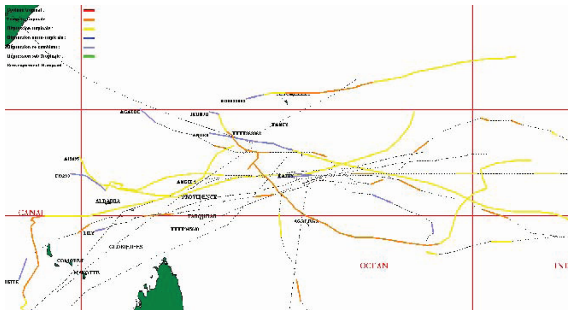
Figure 14: Historical tropical cyclone tracks in the Seychelles EEZ from 1847 to 2003 (Chang-Seng 2005)
