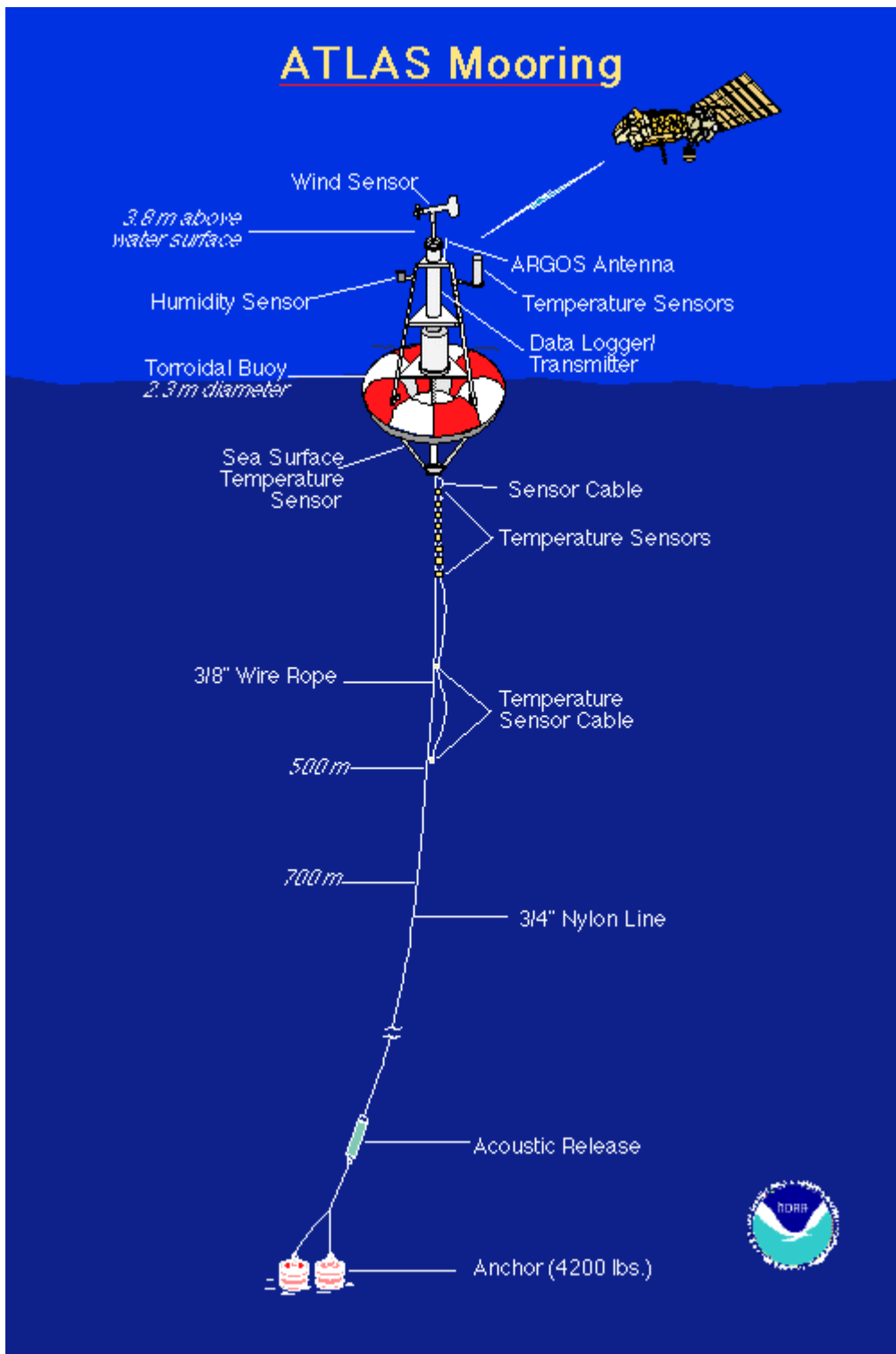
Figure 1: A typical ATLAS mooring array.
